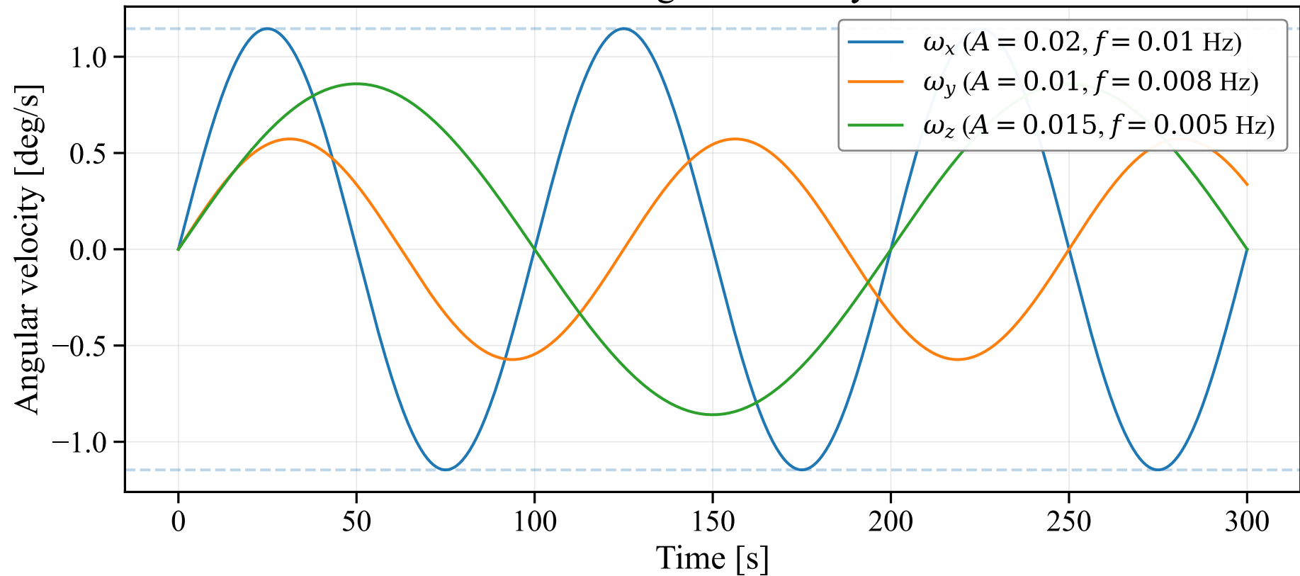
Sinusoidal Angular Velocity Profile
