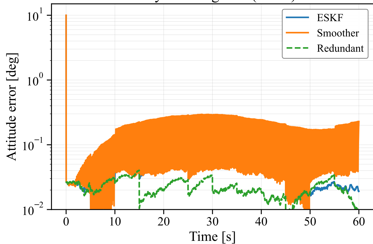
Early Convergence (0-60s)
