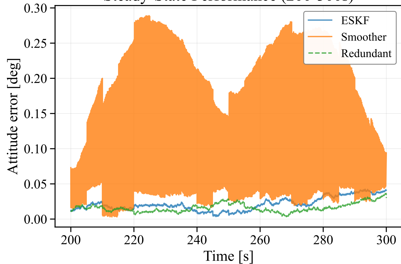
Steady-State Performance (200-300s)
