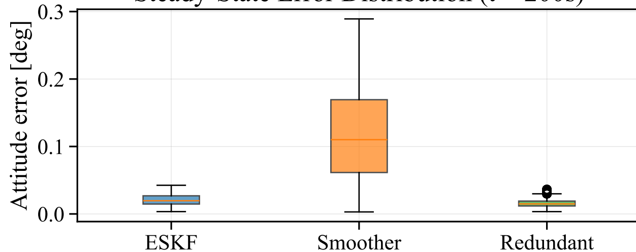
Steady-State Error Distribution (t > 200s)
