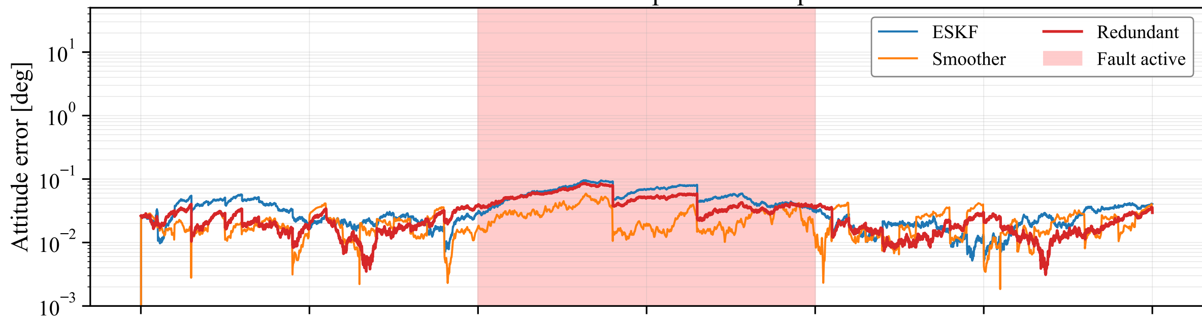
Fault Scenario: Eclipse + ST Dropouts
