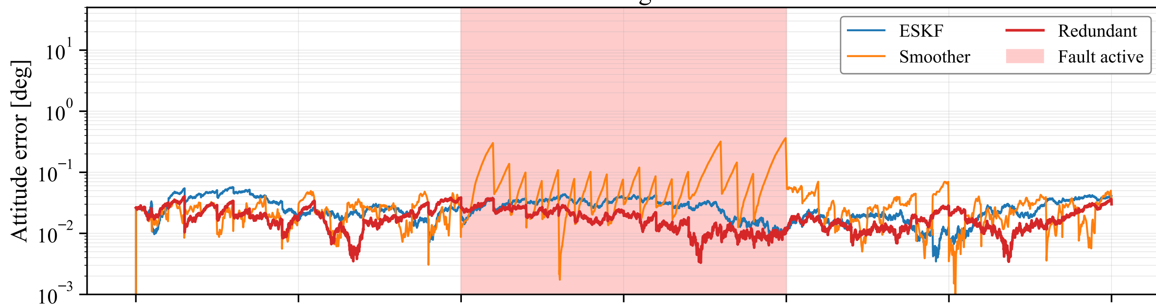
Fault Scenario: Magnetometer Bias
