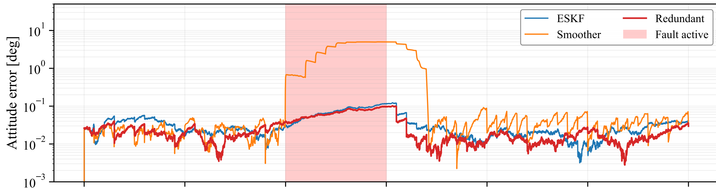
Fault Scenario: Star Tracker Fault
