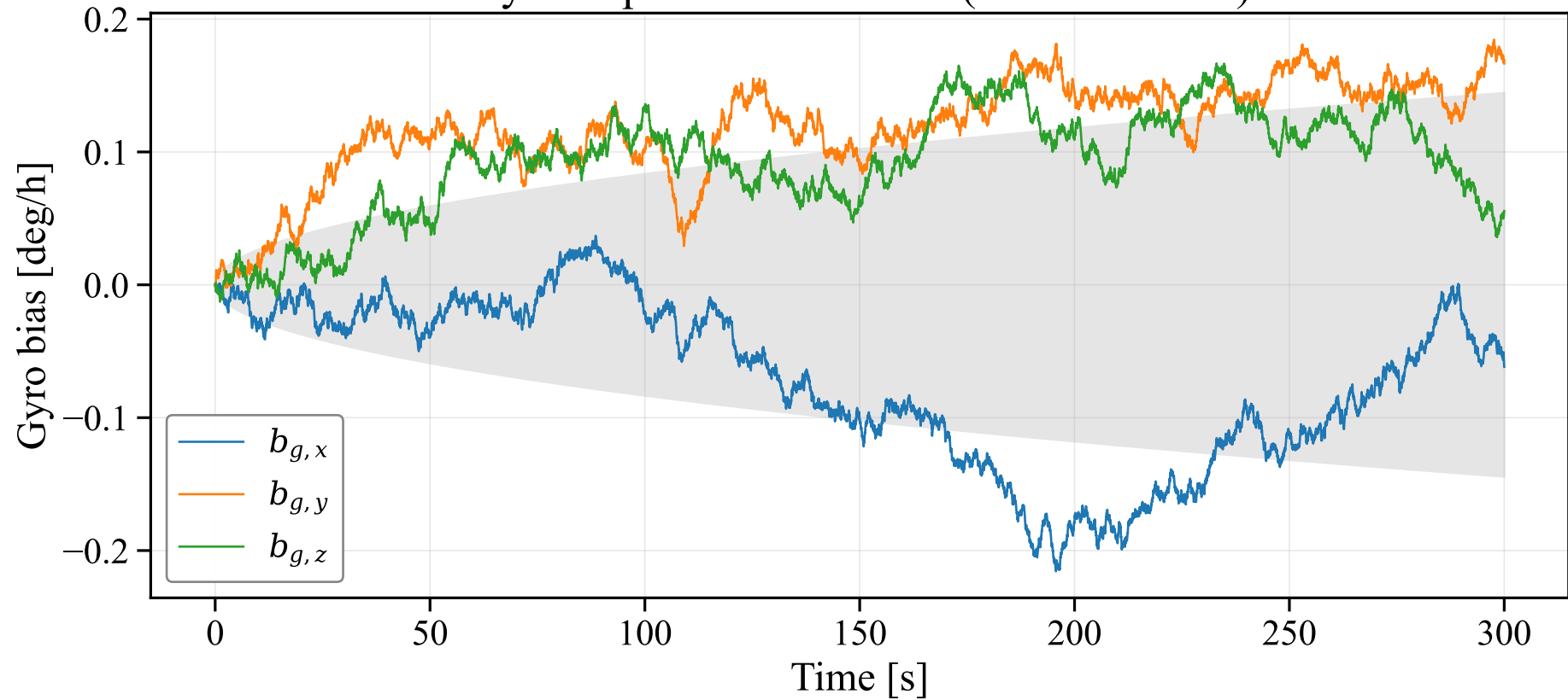
Gyroscope Bias Evolution (Random Walk)
