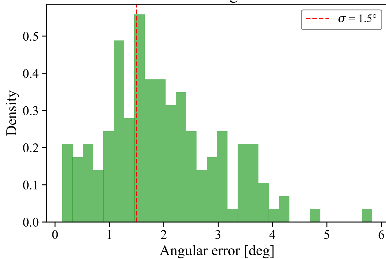
Sun Sensor Angular Error
