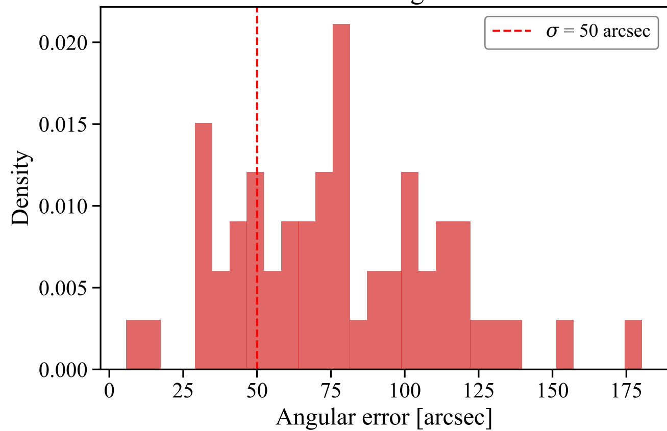
Star Tracker Angular Error
