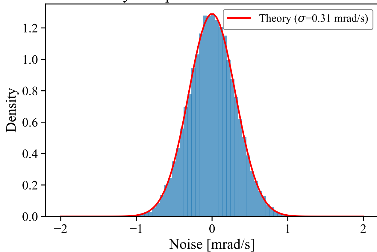
Gyroscope Measurement Noise
