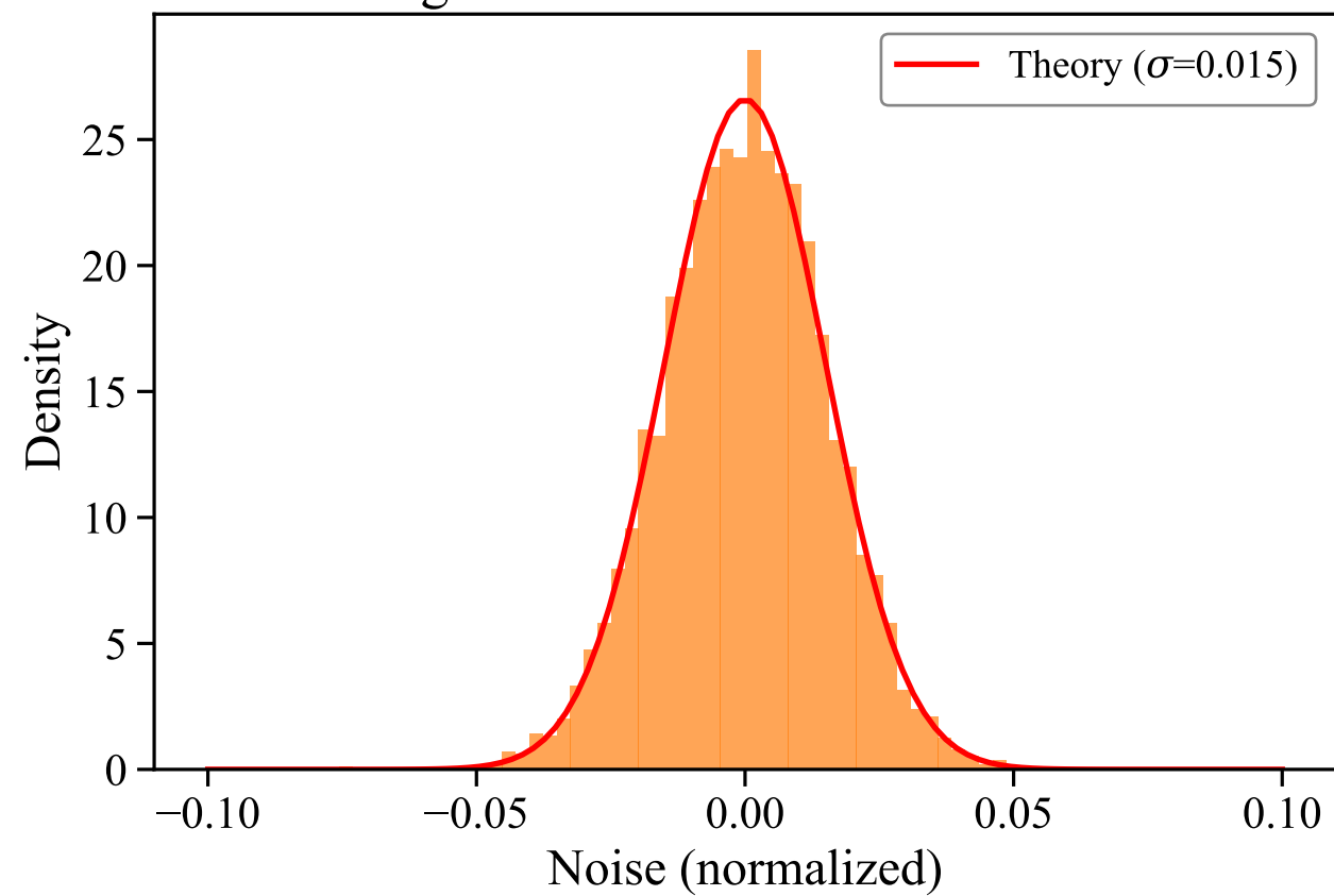
Magnetometer Measurement Noise
