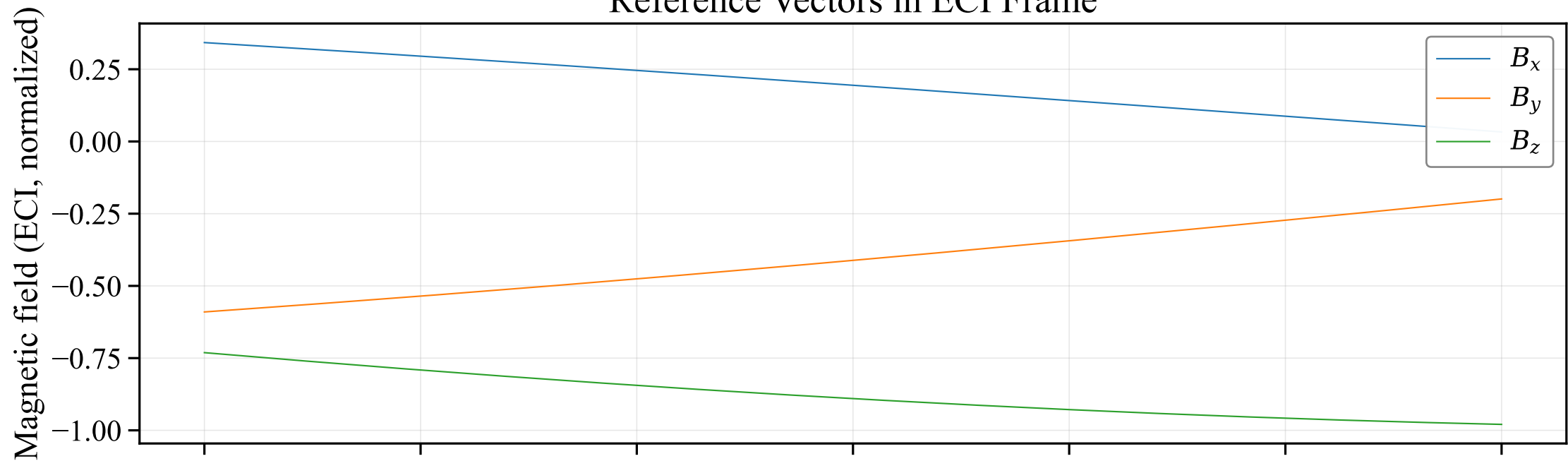
Reference Vectors in ECI Frame
