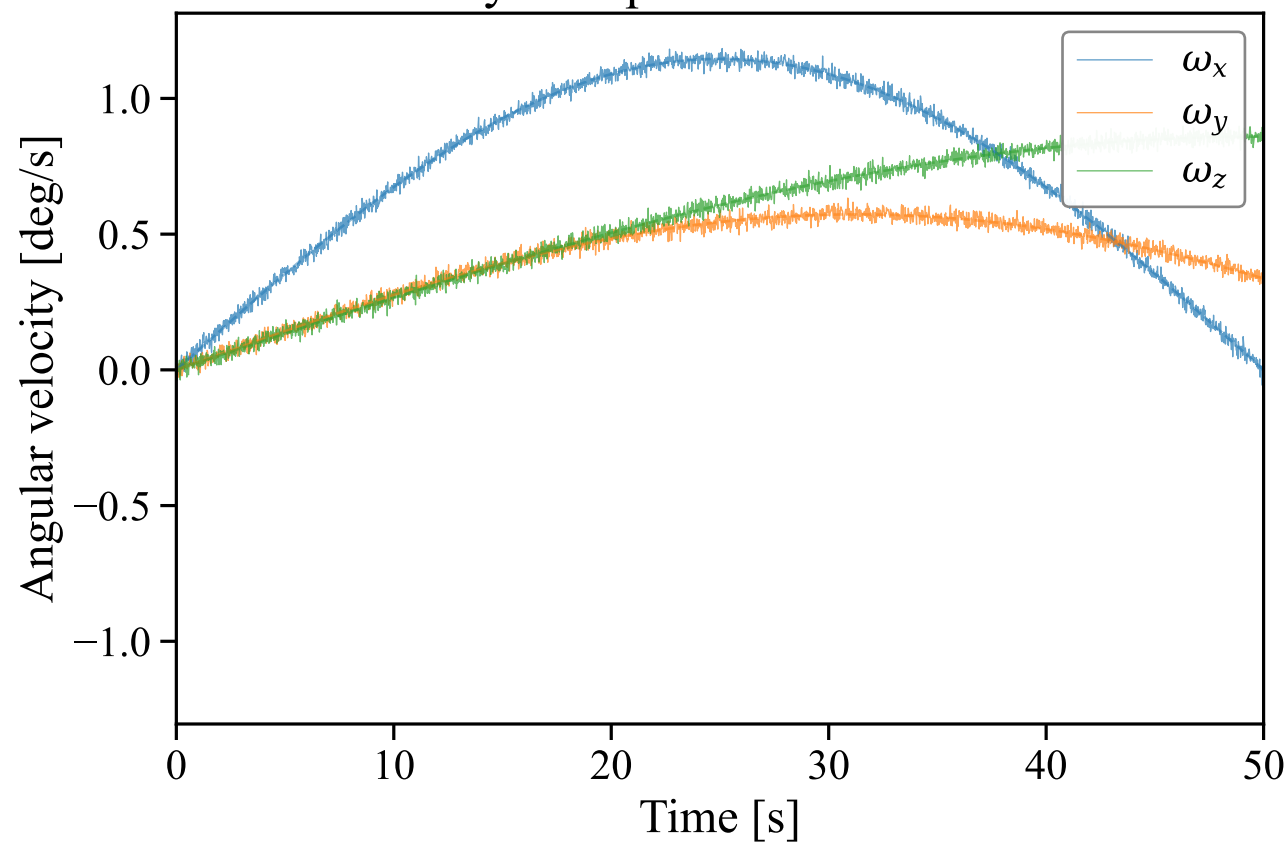
Gyroscope measurements
