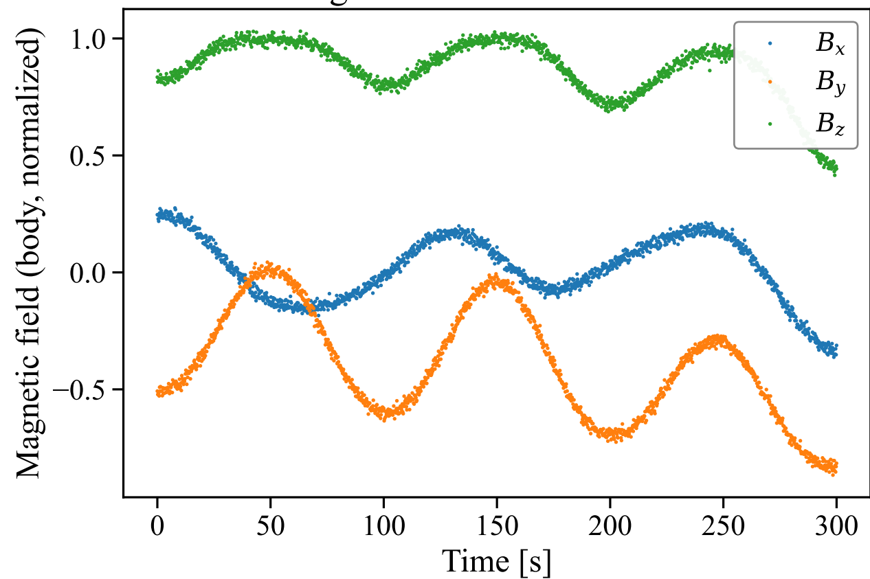
Magnetometer measurements
