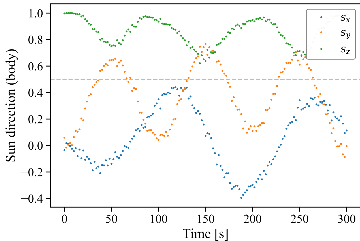
Sun sensor measurements
