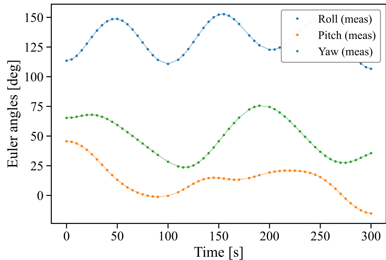
Star tracker measurements
