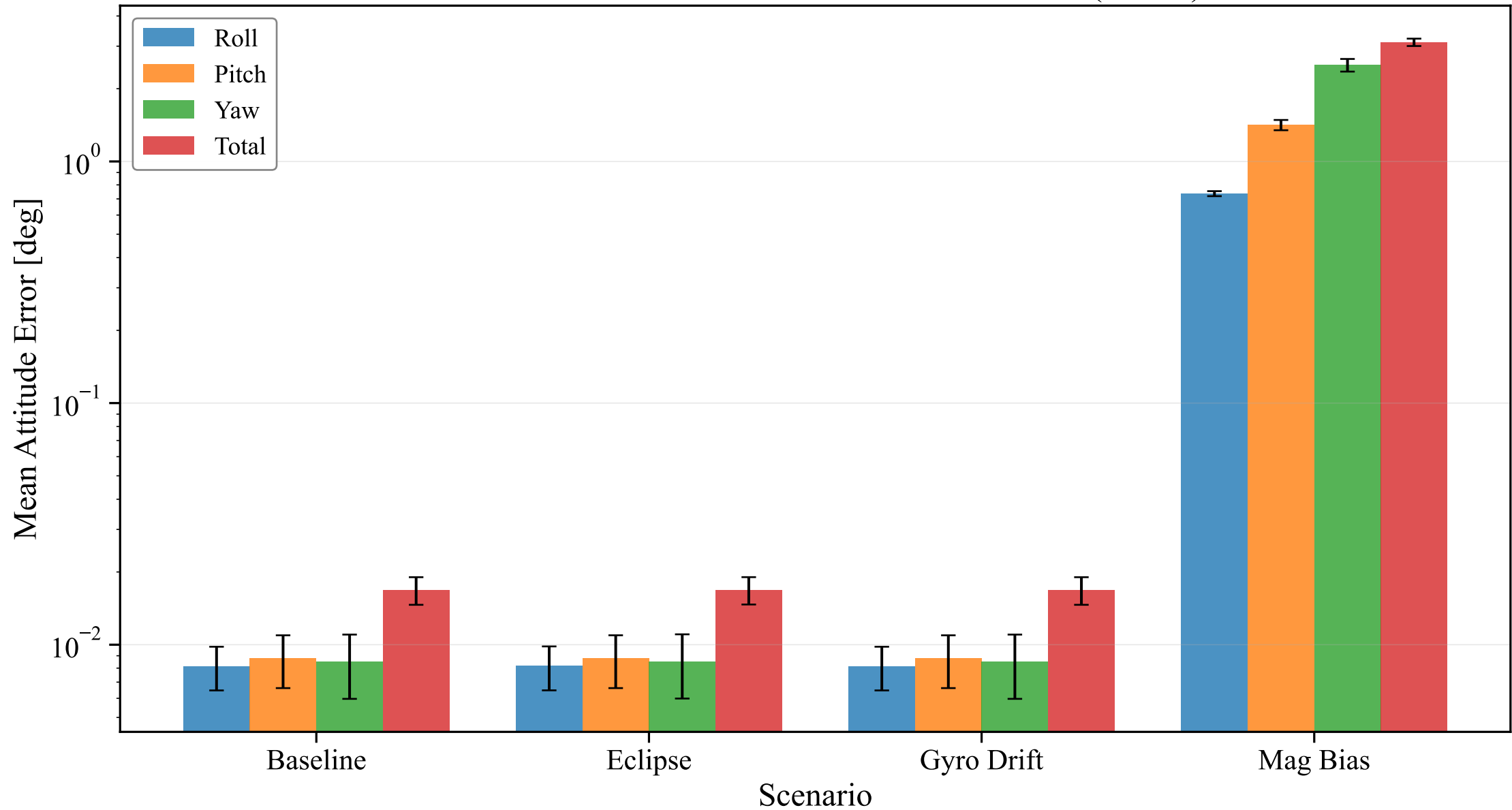
Per-Axis Estimation Errors Across Scenarios (ESKF)
