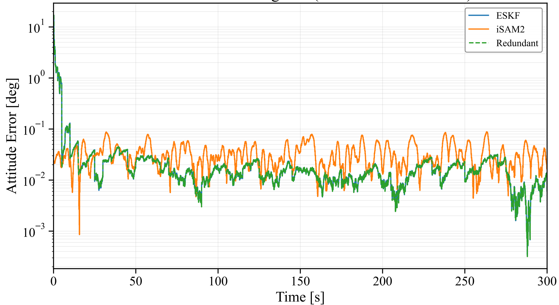
Attitude Error Convergence (Normal Measurements)
