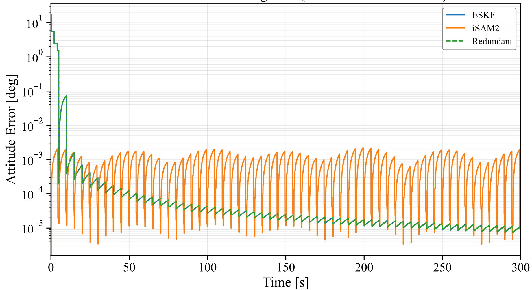
Attitude Error Convergence (Perfect Measurements)
