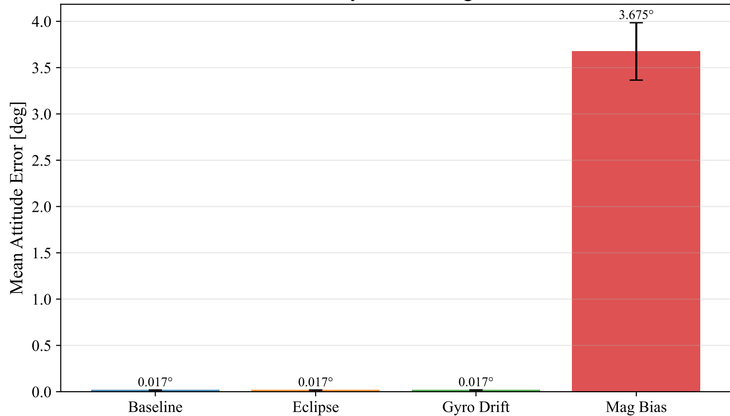
iSAM2 with Cauchy k=0.1 - Degraded Scenarios
