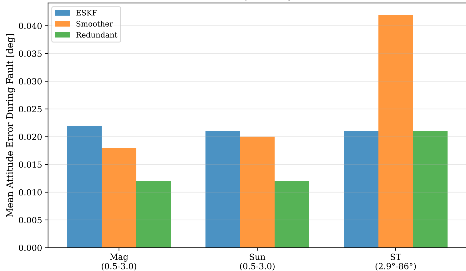
Estimator Accuracy During Sensor Faults
