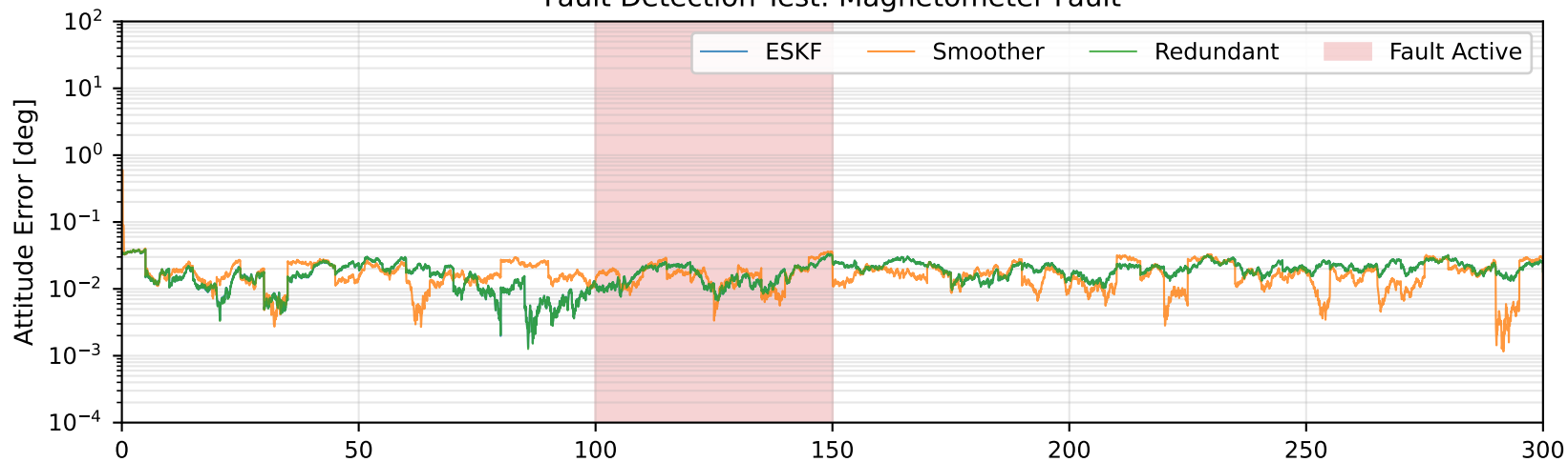
Fault Detection Test: Magnetometer Fault
