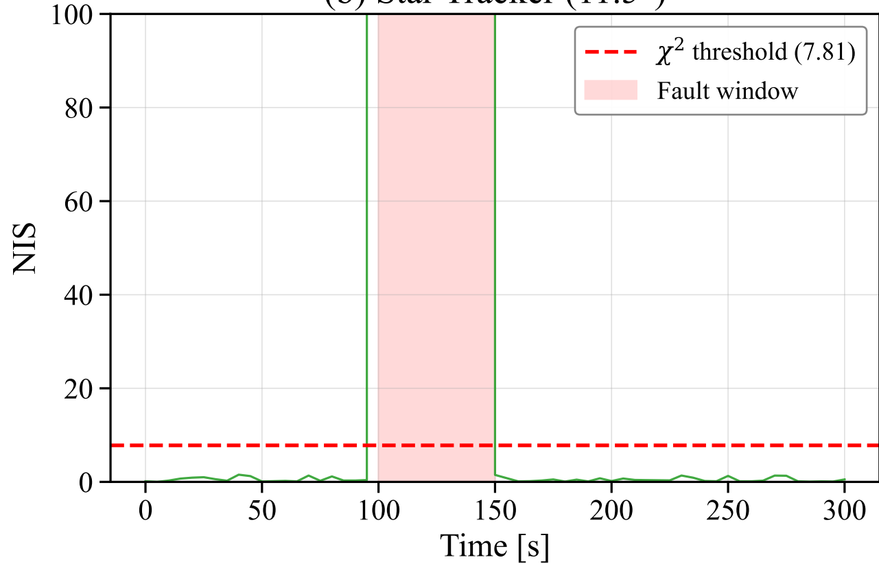
(b) Star Tracker ( 11.5^\circ )
