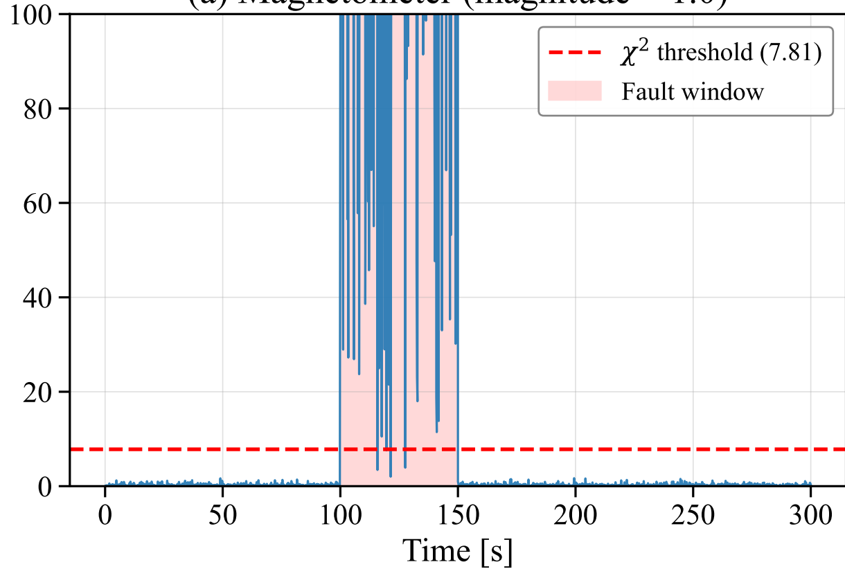
(a) Magnetometer (magnitude = 1.0)
