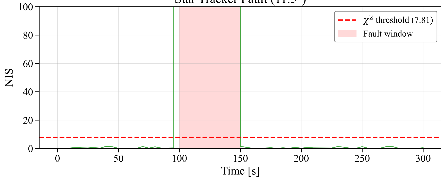
Star Tracker Fault ( 11.5^\circ )
