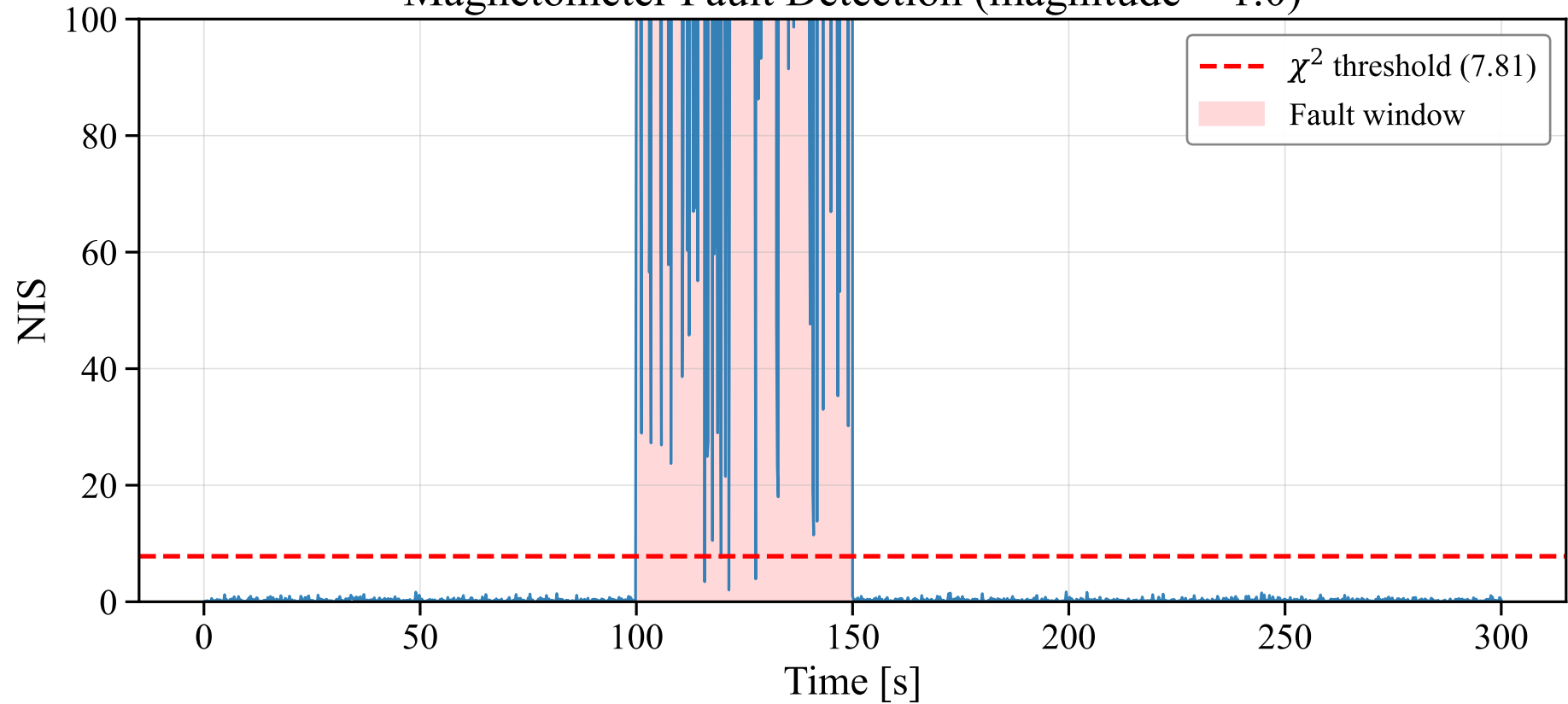
Magnetometer Fault Detection (magnitude = 1.0)
