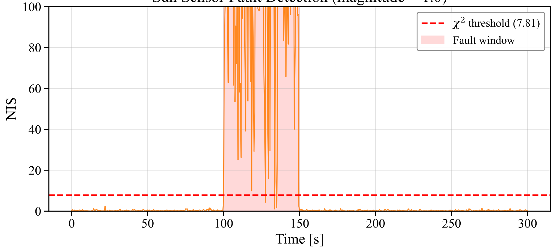
Sun Sensor Fault Detection (magnitude = 1.0)
