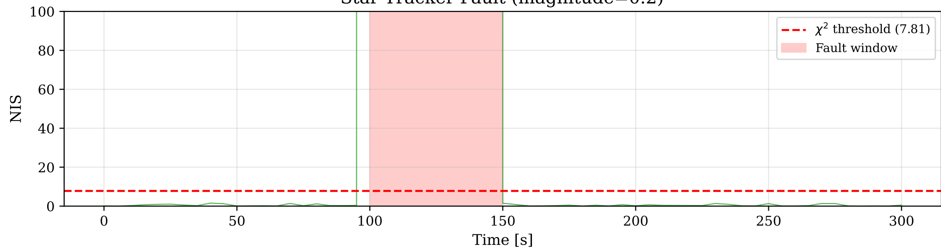
Star Tracker Fault (magnitude=0.2)
