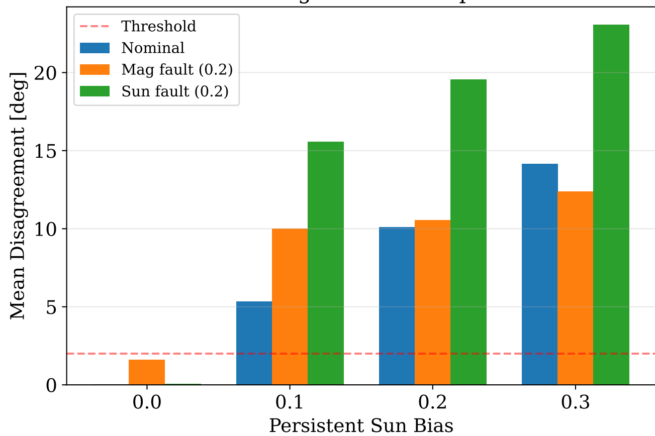
Mean Disagreement Comparison
