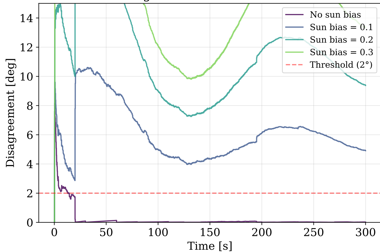
Additional Sun Fault (bias=0.2) Detection
