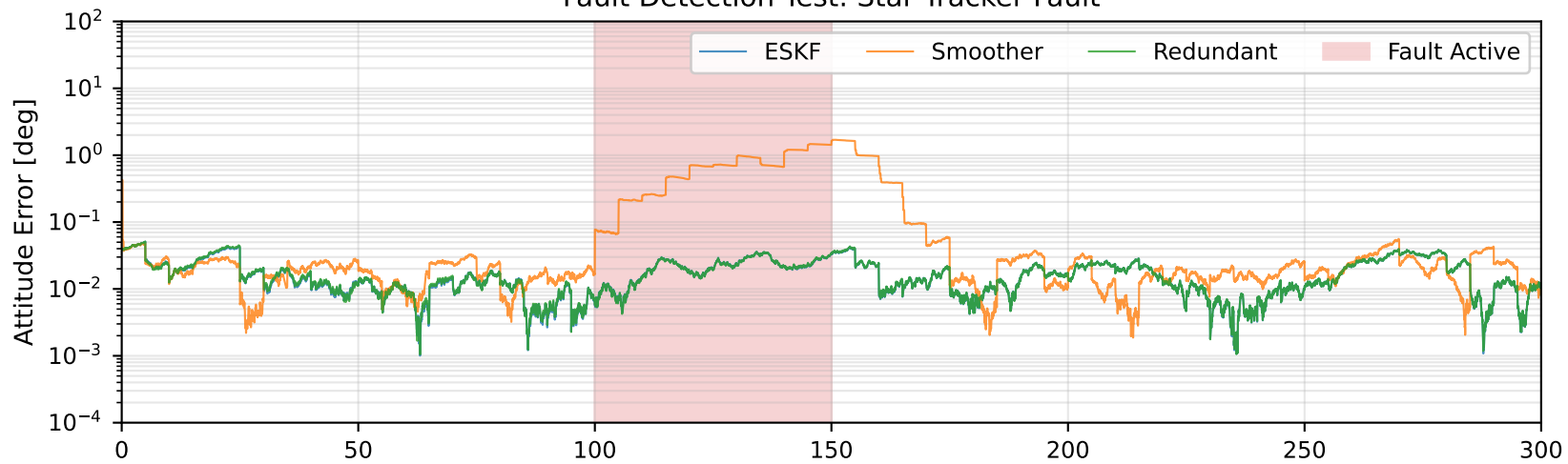
Fault Detection Test: Star Tracker Fault
