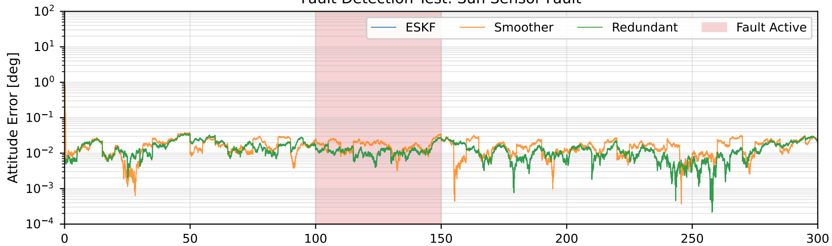
Fault Detection Test: Sun Sensor Fault
