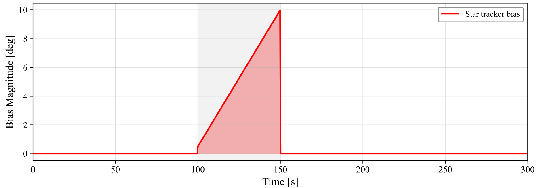
Star Tracker Fault Profile
