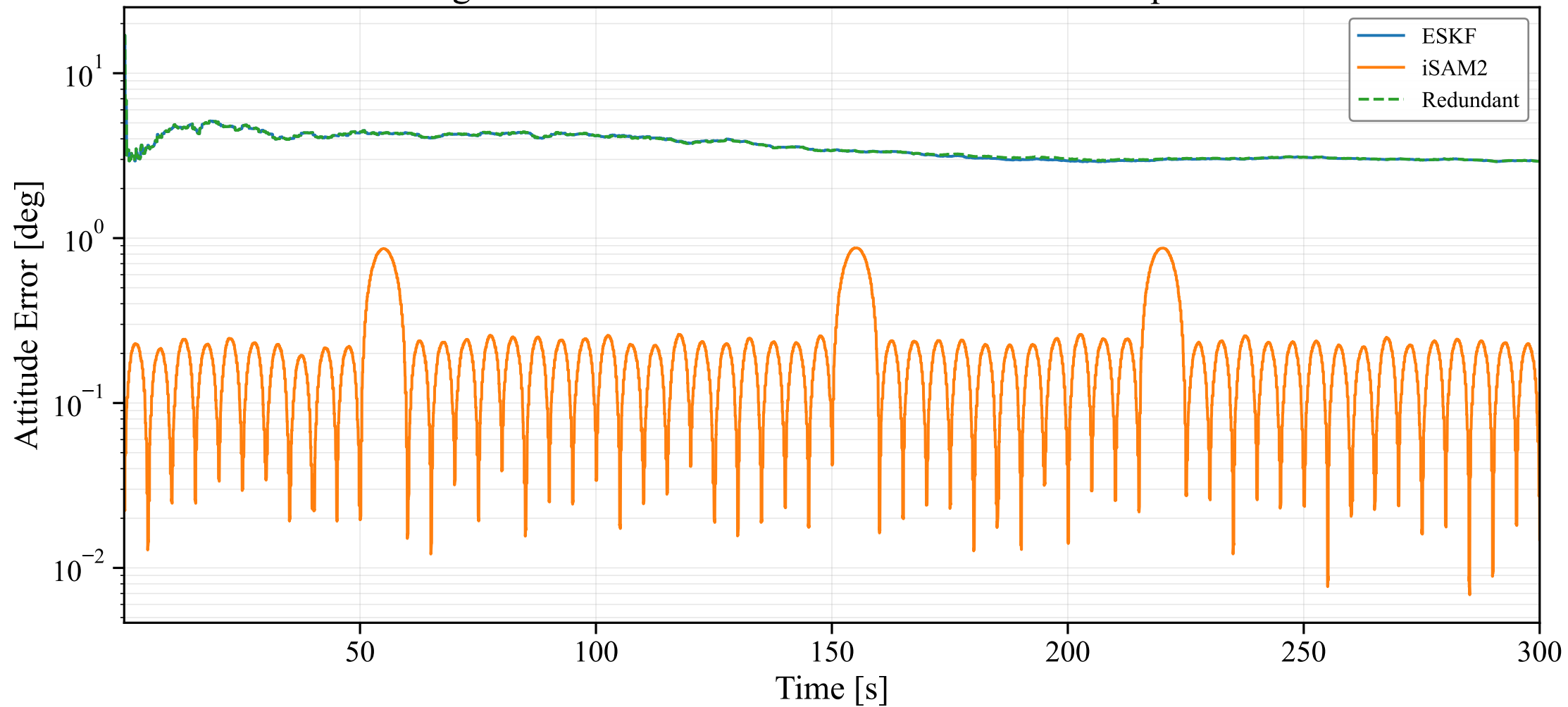
Magnetometer Bias Scenario: Attitude Error Comparison
