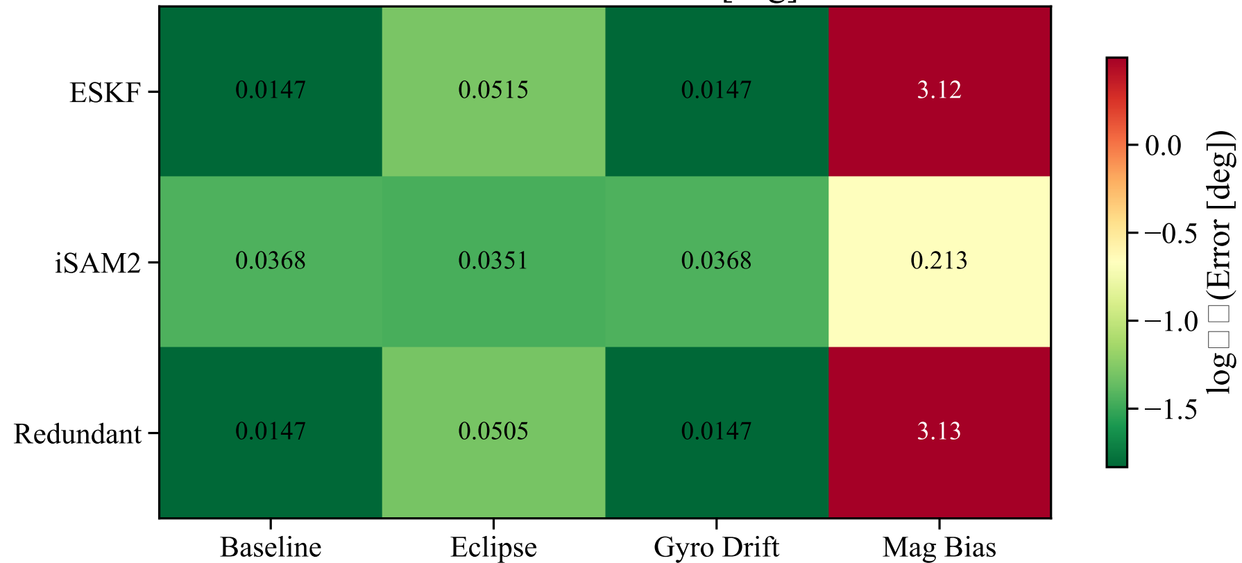
Mean Attitude Error [deg]
