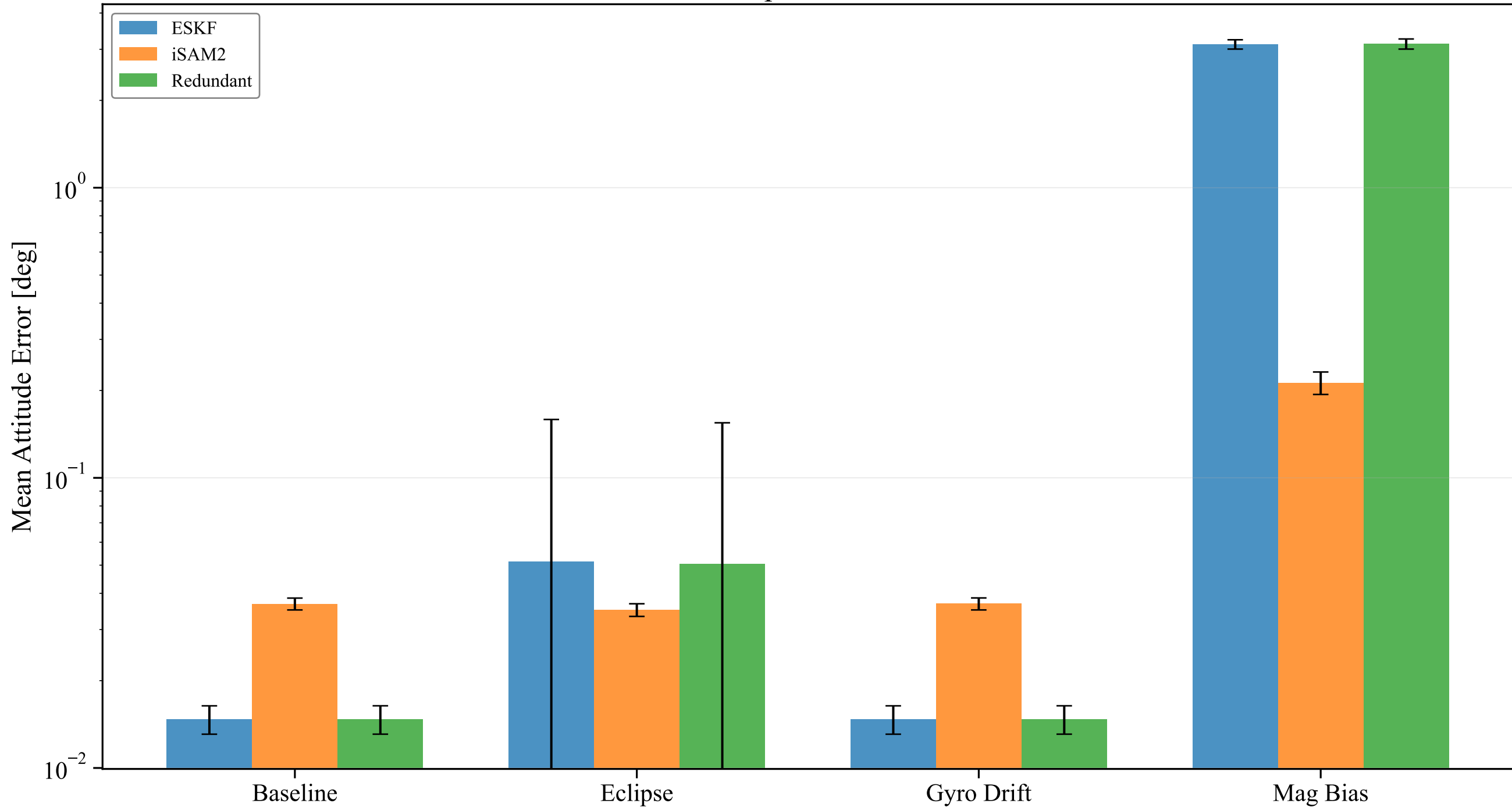
Monte Carlo Comparison Across Scenarios
