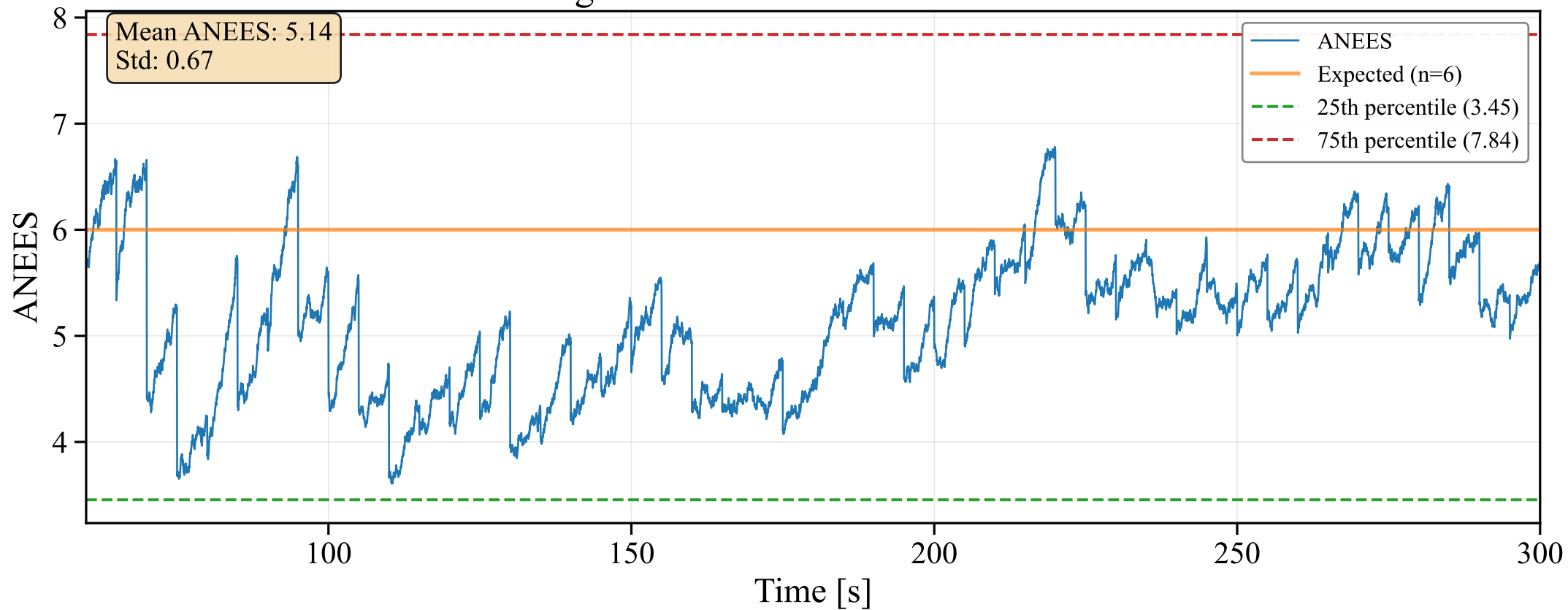
Average NEES over 20 Monte Carlo Runs
