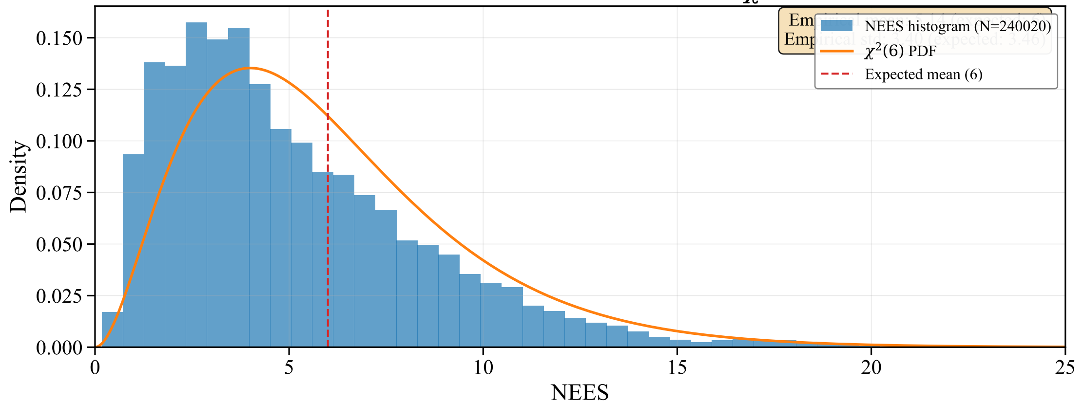
NEES Distribution vs Theoretical \chi^2
