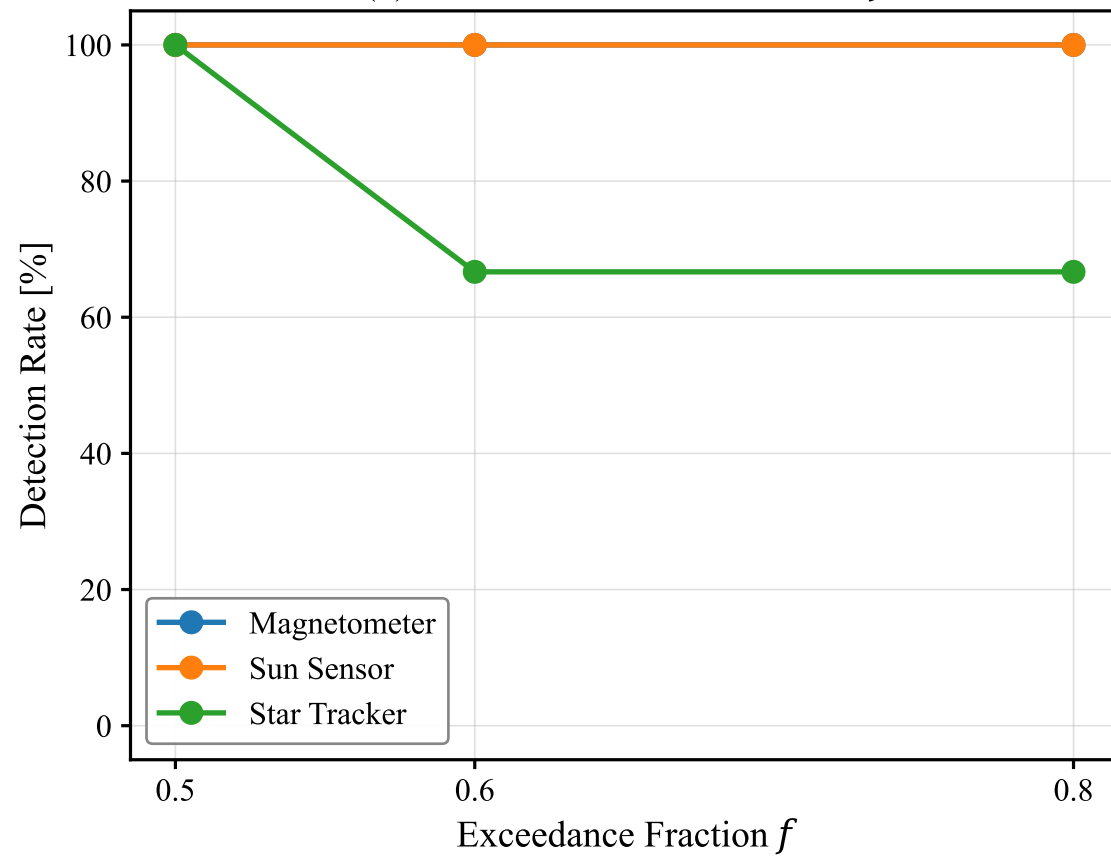
(a) ESKF: Detection Rate vs. f
