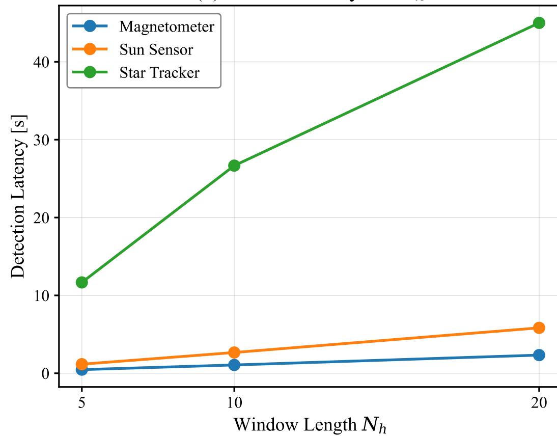
(b) ESKF: Latency vs. N_h
