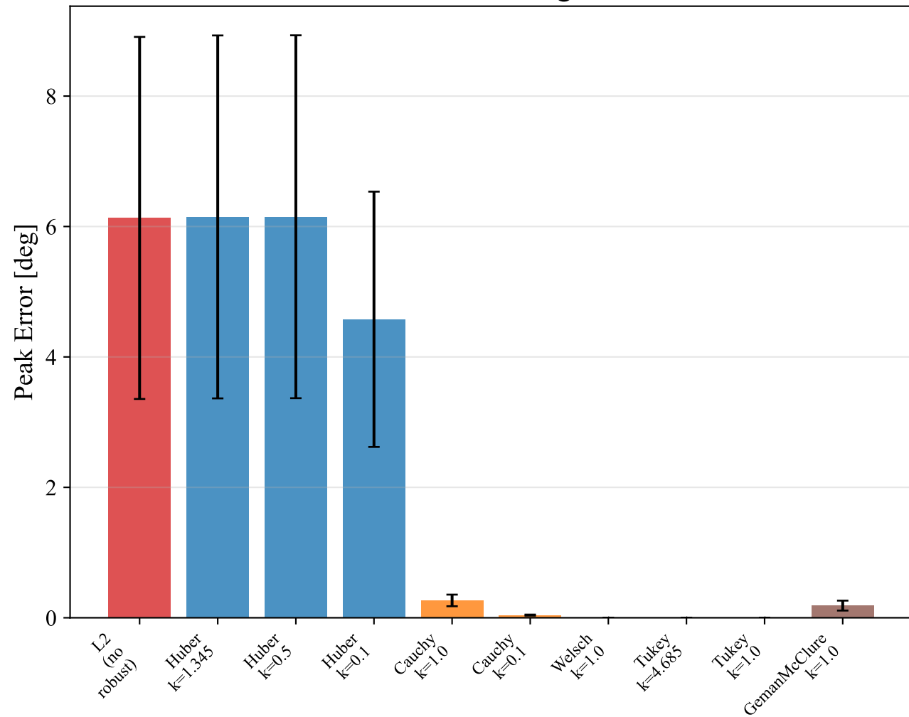
Peak Error During Fault
