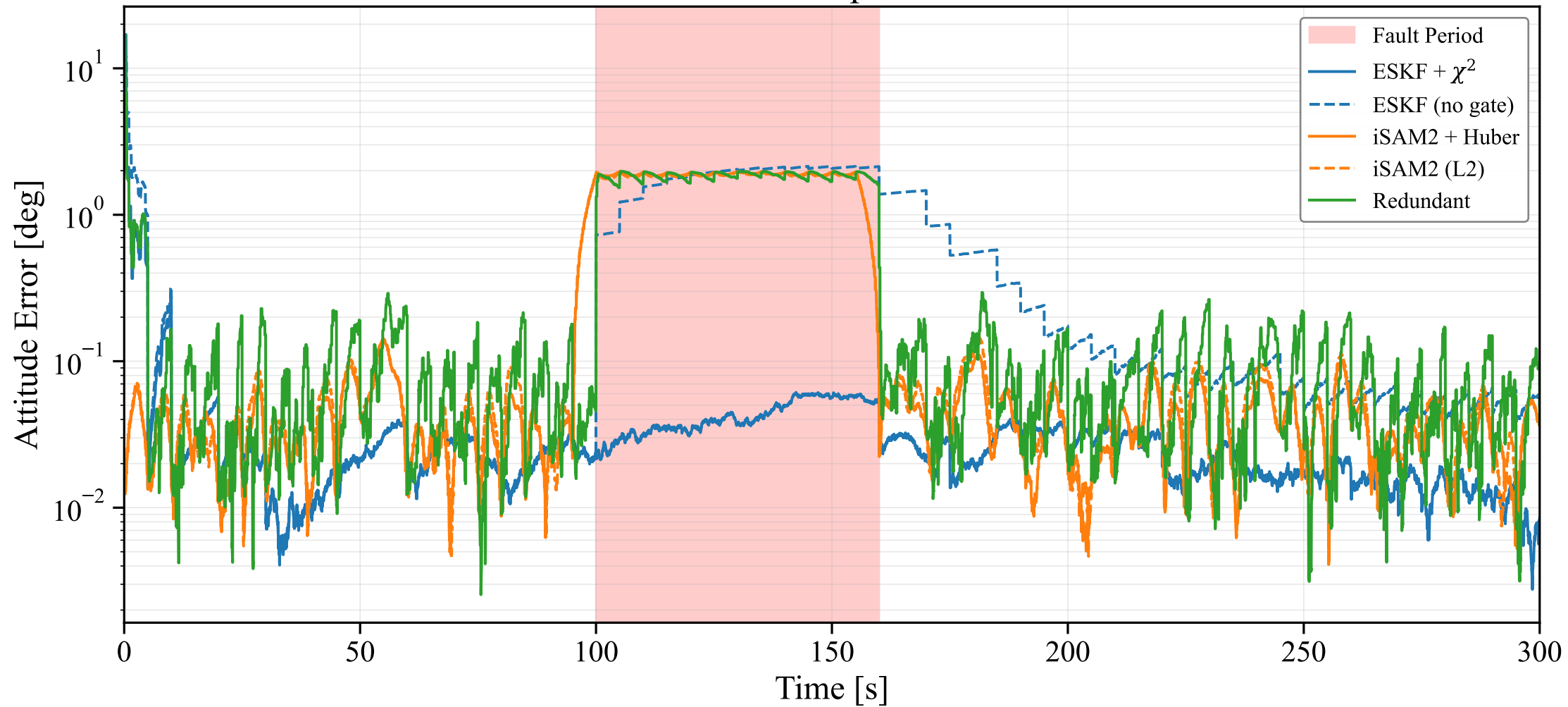
Robustness Mechanism Comparison: Star Tracker Fault
