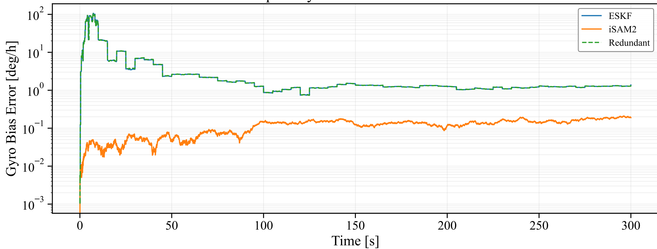
Eclipse: Gyro Bias Estimation Error
