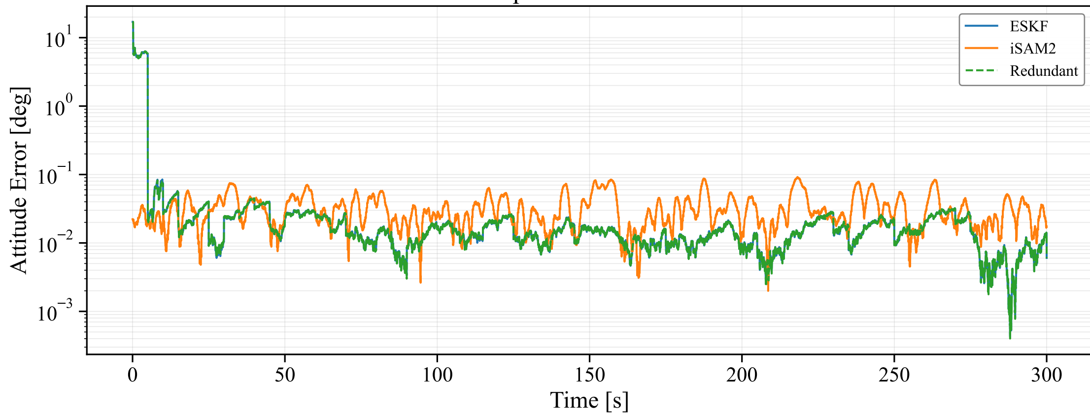
Eclipse: Attitude Error
