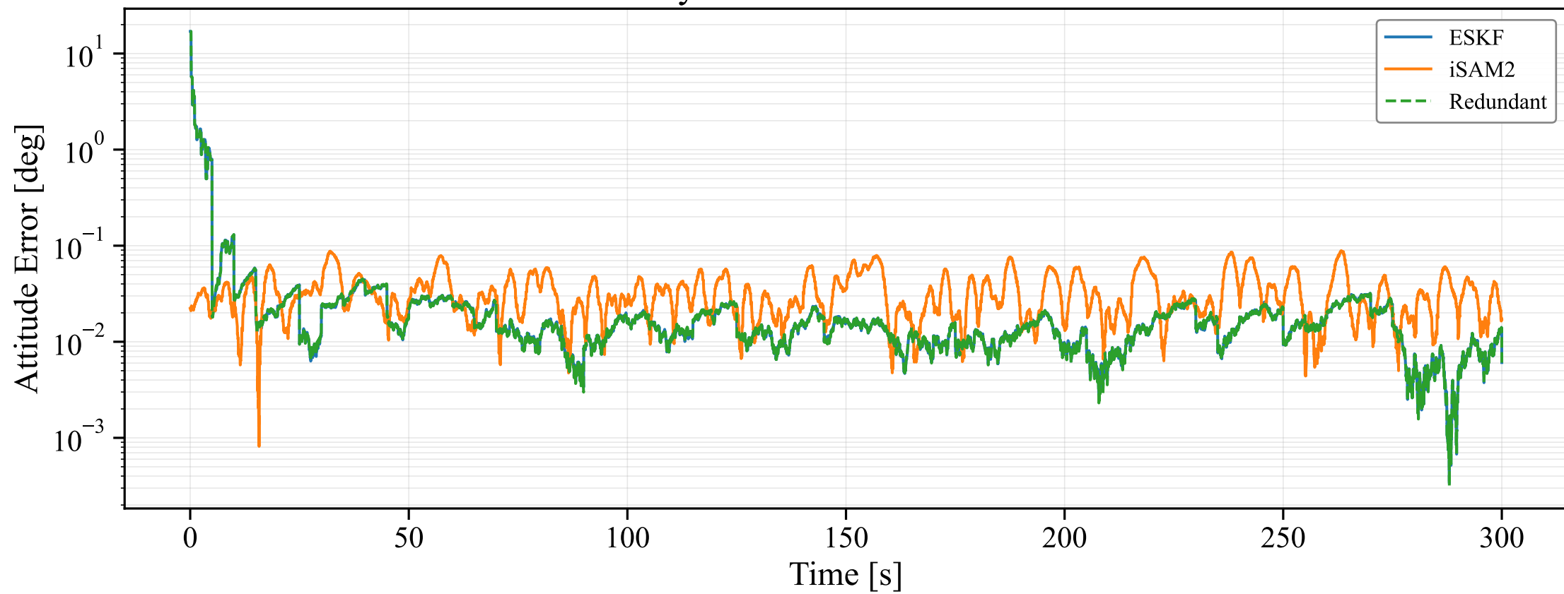
Gyro Drift: Attitude Error
