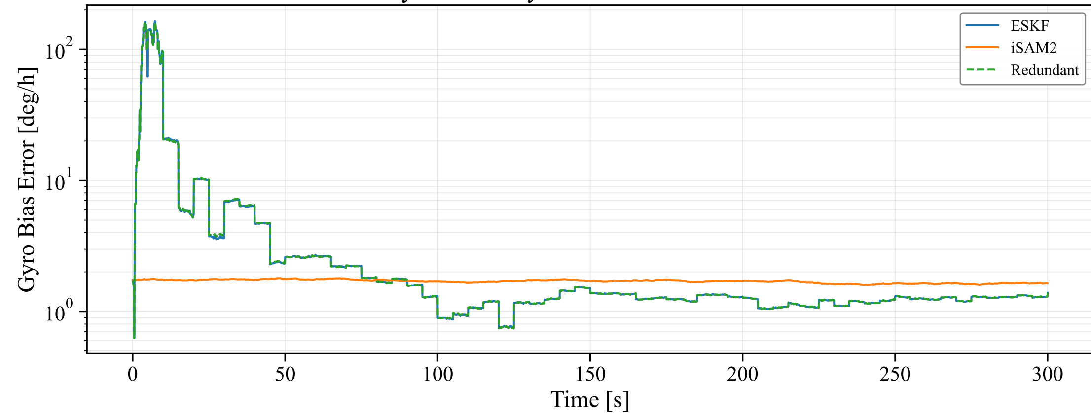
Gyro Drift: Gyro Bias Estimation Error
