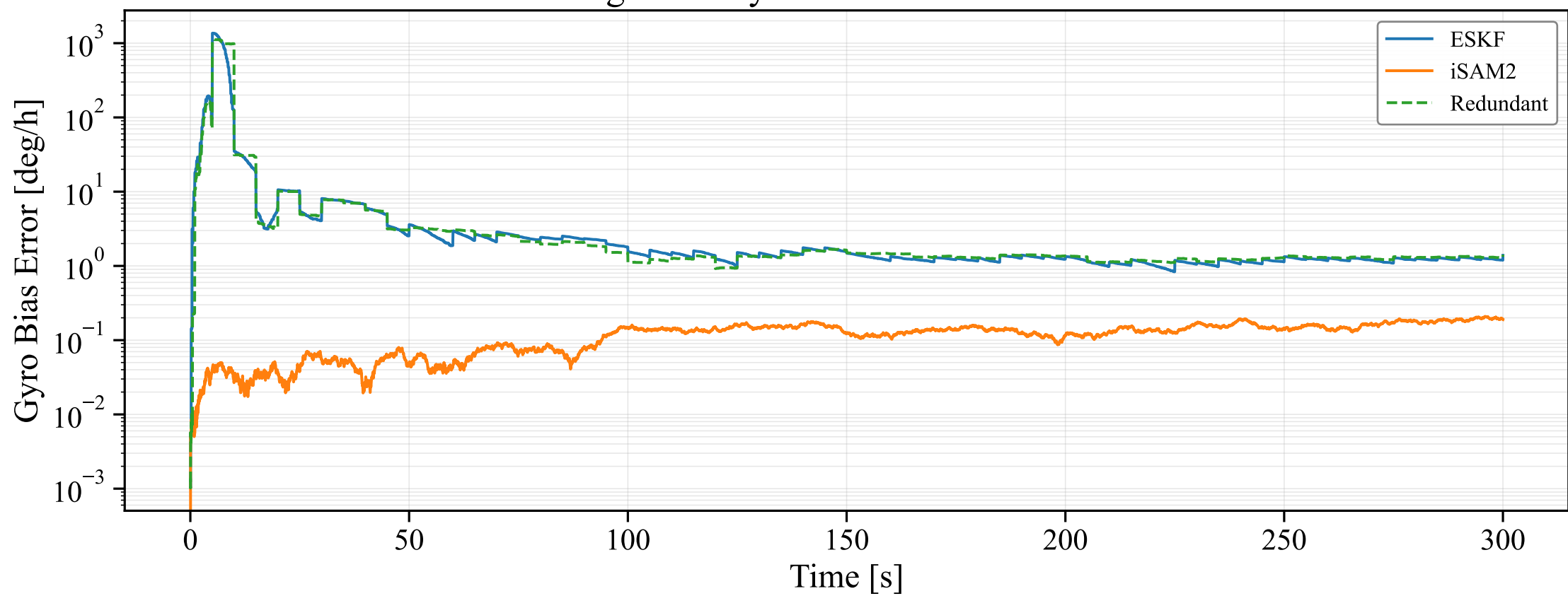
Mag Bias: Gyro Bias Estimation Error
