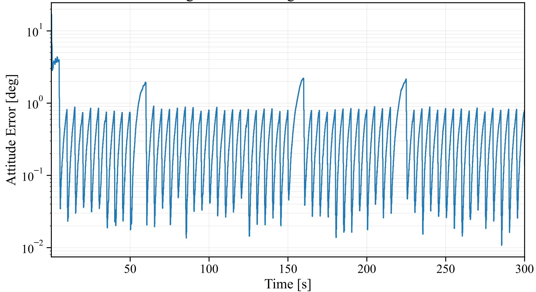
Fixed-Lag Smoother: Magnetometer Bias Scenario
