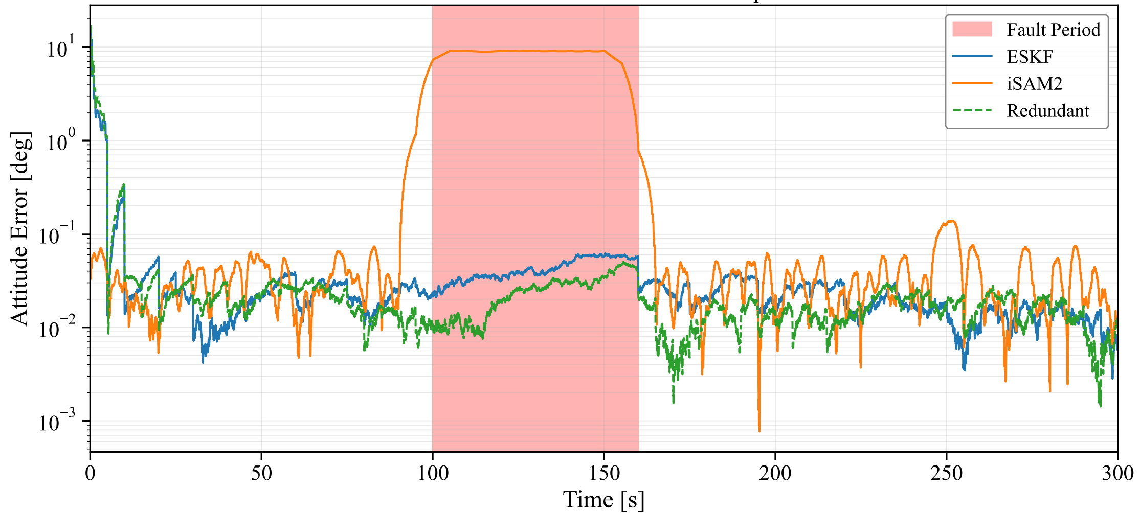
Star Tracker Transient Fault: Example Run
