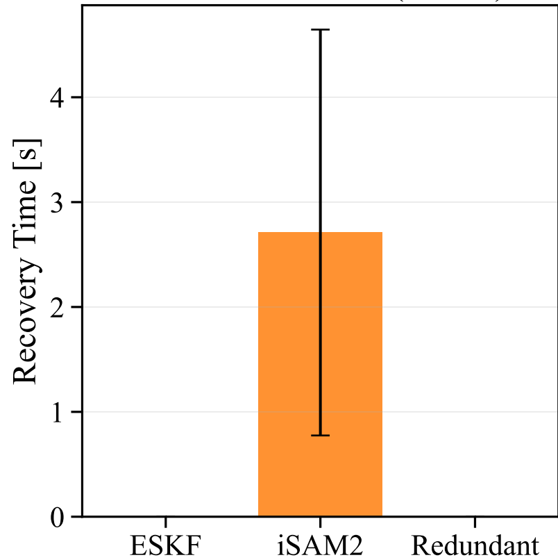
Time to Recover ( <0.1^\circ )
