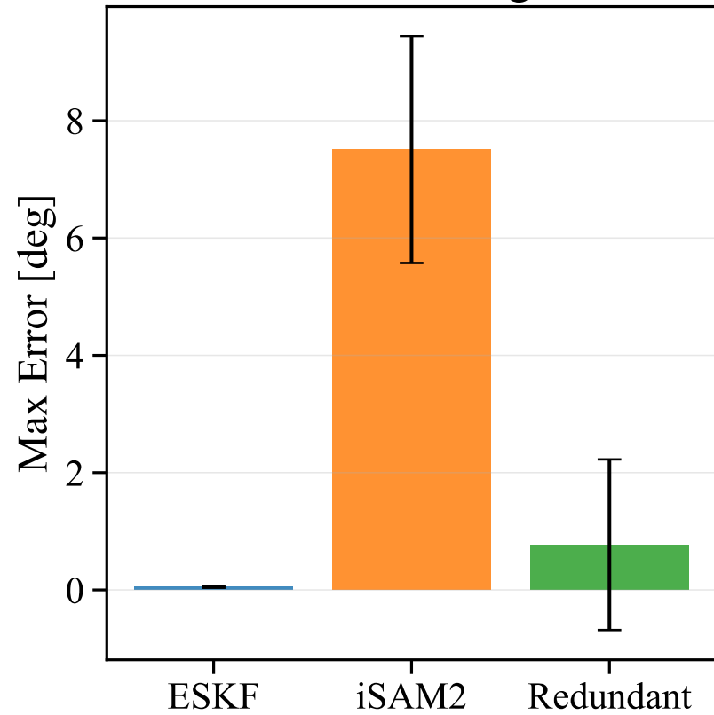
Peak Error During Fault
