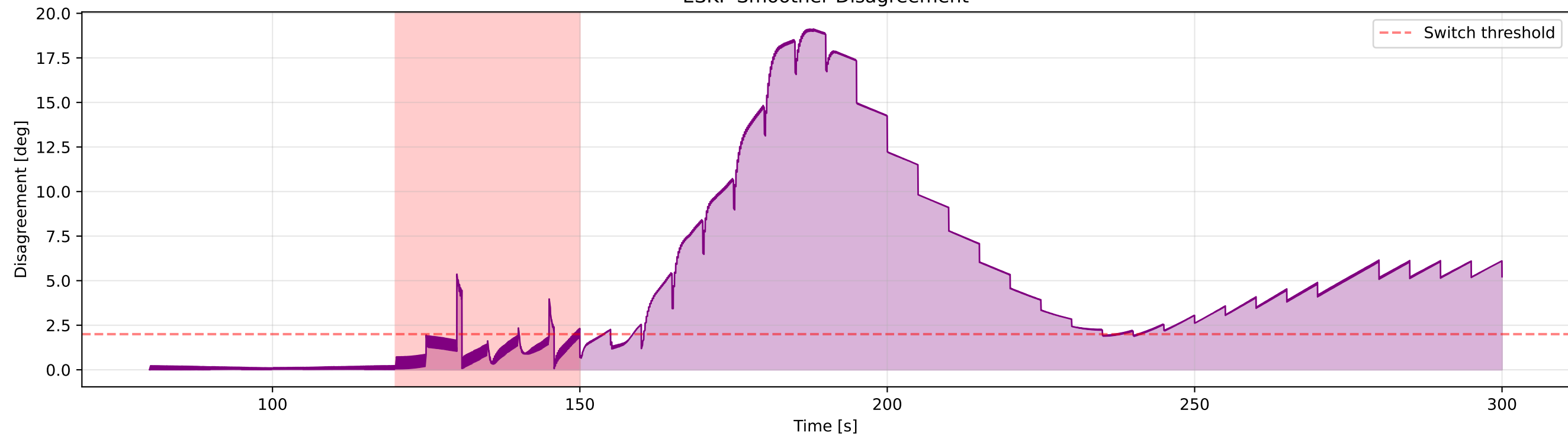
ESKF-Smoother Disagreement
