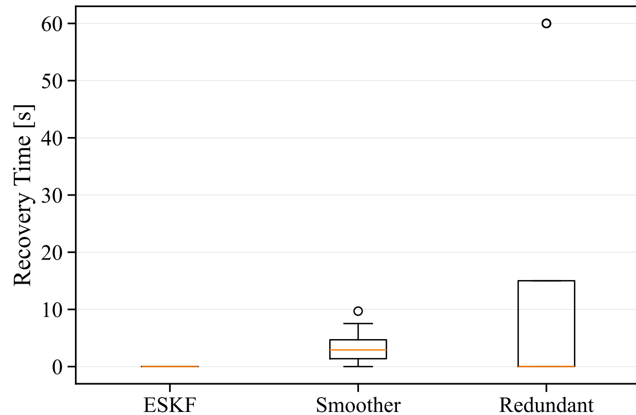
Time to Recover Below 0.05^\circ
