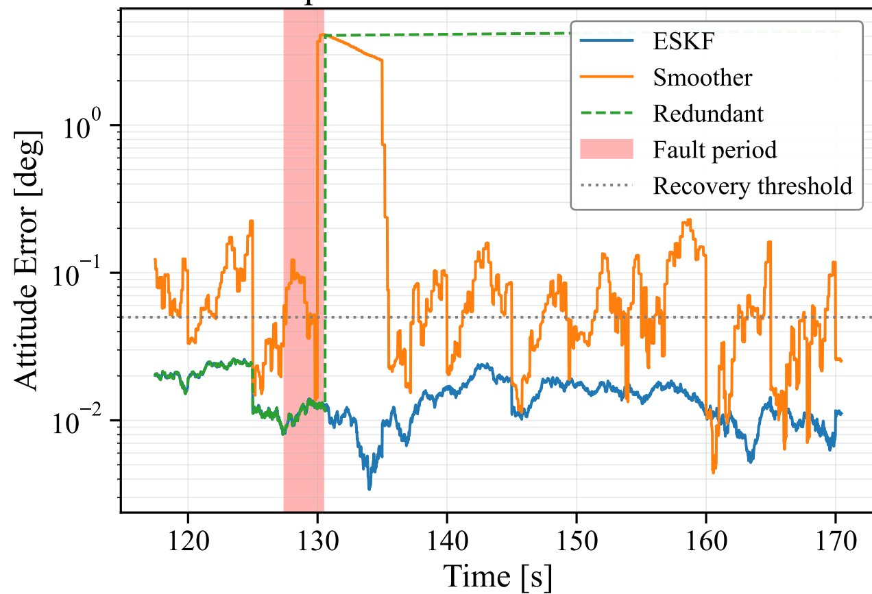
Example: Transient Star Tracker Fault
