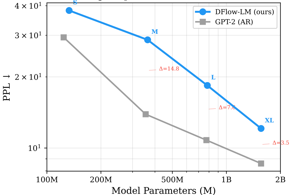
Scaling: Gap Narrows with Model Size
