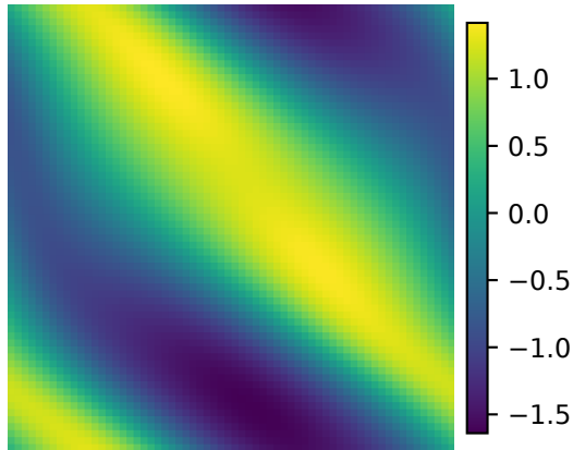
Ground truth
