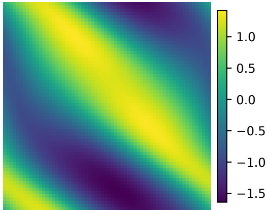
Prediction
