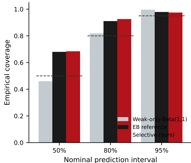
c Interval coverage
