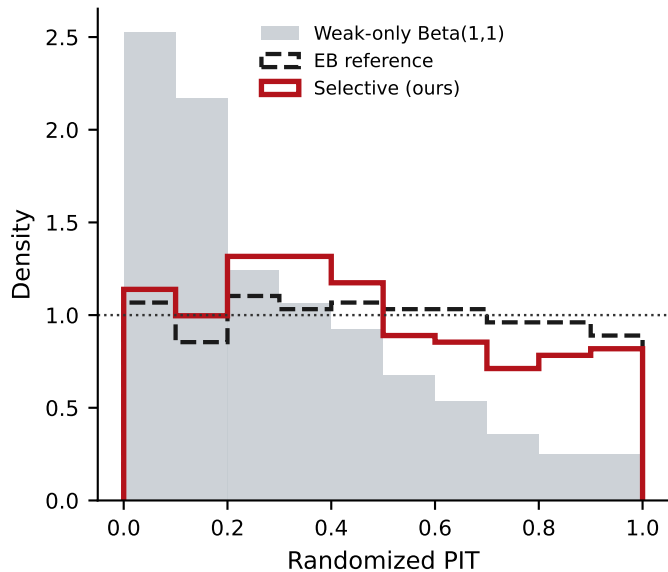
a PIT uniformity
