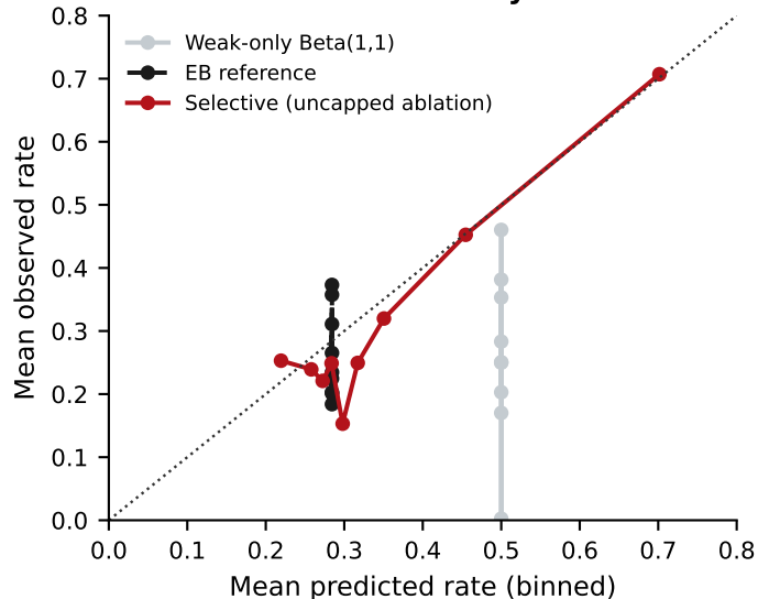
b Reliability
