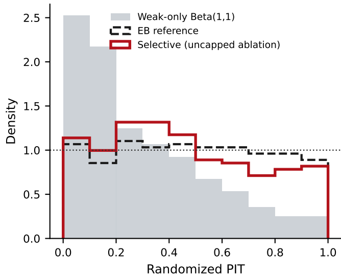
a PIT uniformity
