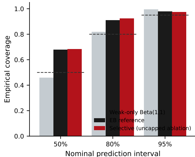
c Interval coverage
