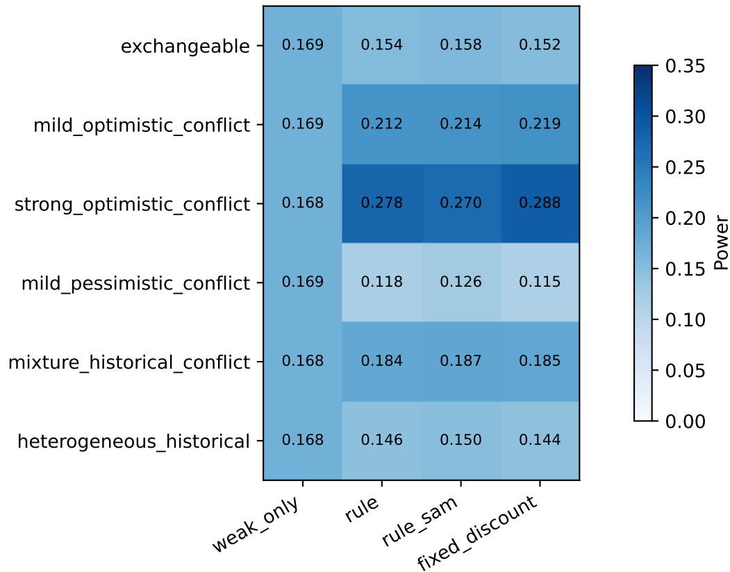
Simulation operating characteristics: empirical power
