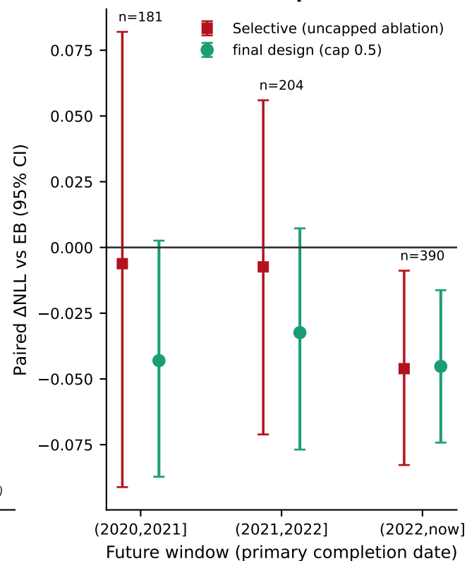
b Per-window paired delta
