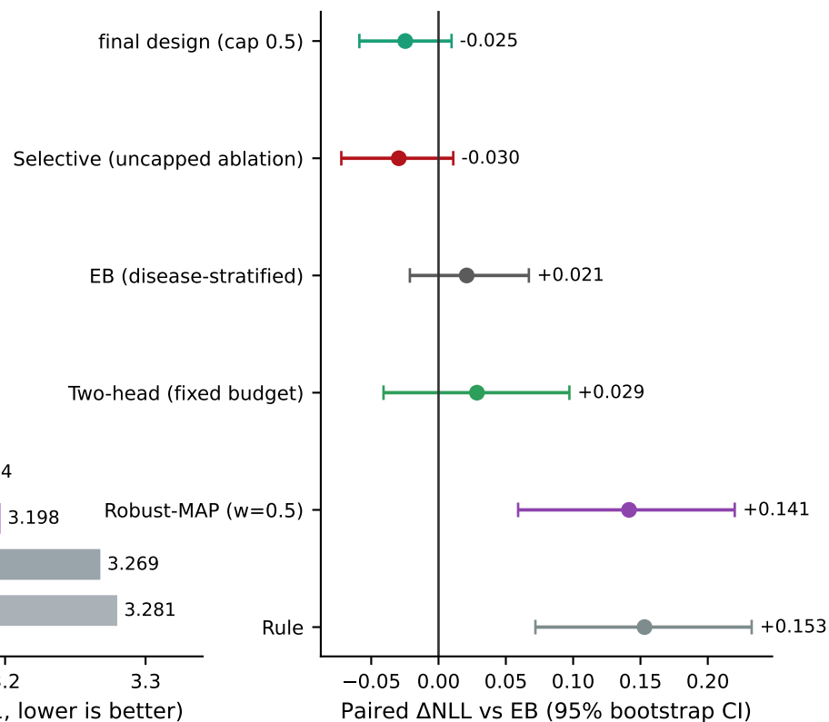
b Paired deltas vs EB
