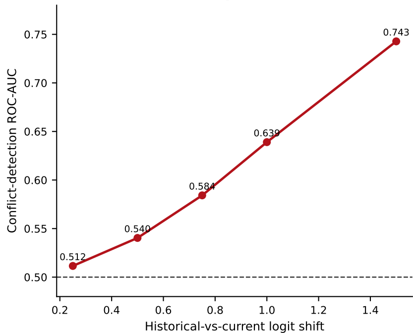
b SAM detects prior-data conflict
