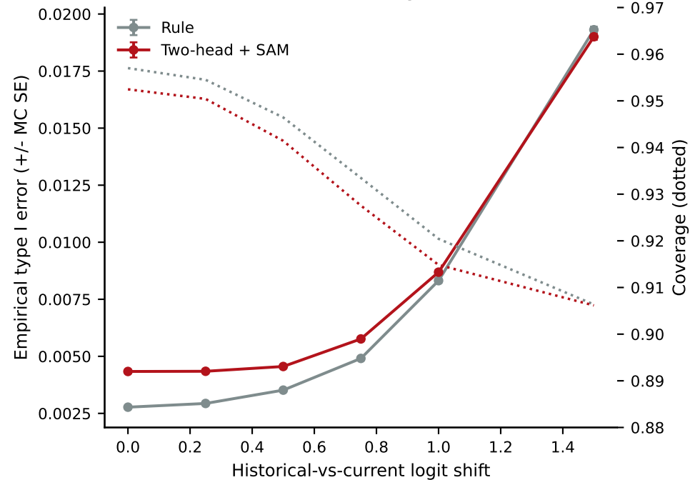
a Conflict safety curve
