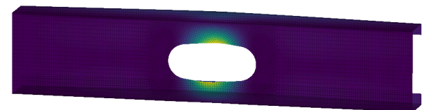
Figure 5: Lowest buckling mode localized at a service hole (web strips beside the hole), 5 mm mesh (top) and 2.5 mm mesh (bottom).
