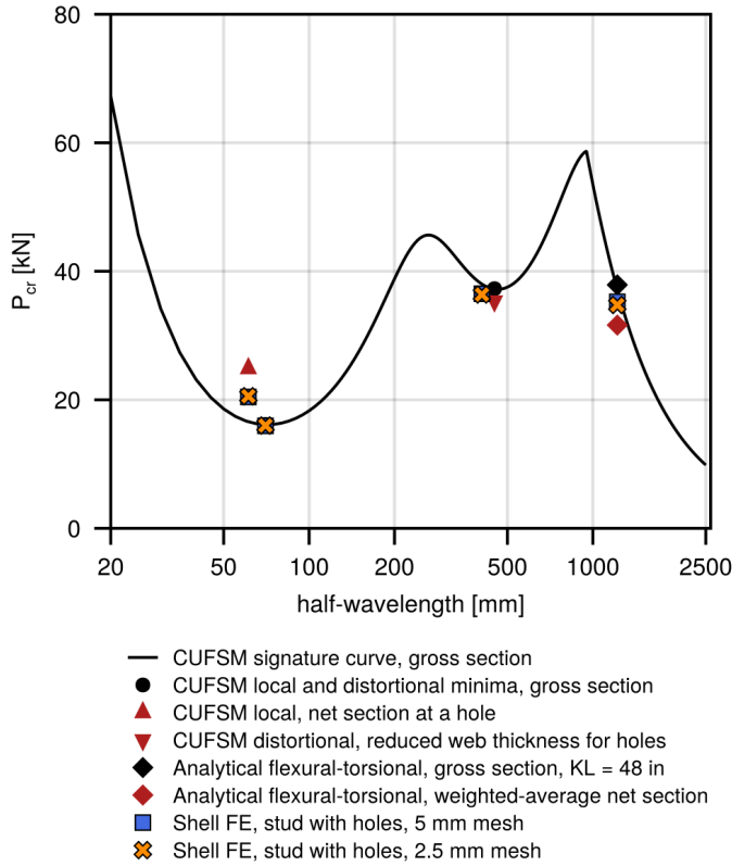
Figure 3: Finite strip signature curve of the gross section with the hole approximations, the analytical global loads for KL = 48 in, and the shell finite element results for the perforated stud, plotted at the half-wavelength of the corresponding reference value (global modes at 1219 mm).
