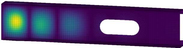
5 mm mesh, 15.95 kN (3.59 kips), z = 0–460 mm
