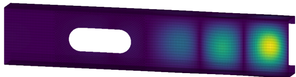
Figure 4: Lowest local buckling mode, close-up around the region of largest displacement, 5 mm mesh (top) and 2.5 mm mesh (bottom).
