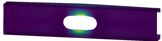
5 mm mesh, 20.45 kN (4.60 kips), z = 1904–2364 mm
