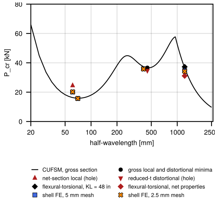
Figure 3: Finite strip signature curve of the gross section with the hole approximations, the analytical global loads for KL = 48 in, and the shell finite element results for the perforated stud, plotted at the half-wavelength of the corresponding reference value (global modes at 1219 mm).
